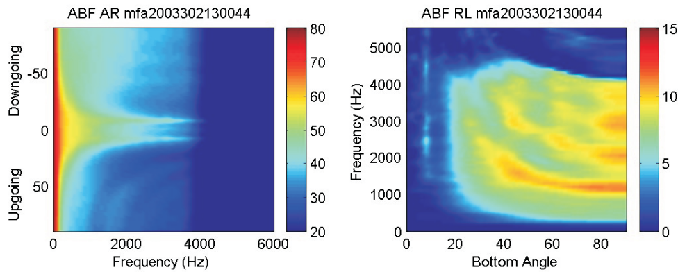
FIGURE 6. Directionality of ambient noise (left) for the northern site. Bottom reflectivity derived by processing the ambient noise (right).
